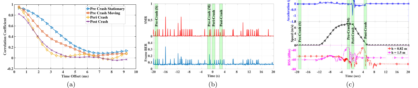
Fig. 11. (a) Channel coherence in the 4 interested intervals of bogie test, (b) BER and symbol missing rate (SMR) of every 5 frames in bogie test, (c) Acceleration, velocity, and RSS on two co-located receivers in sedan test.
