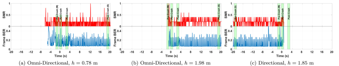
Fig. 23. BER and symbol missing rate (SMR) of every 5 frames for barrier antennas in pickup test.
