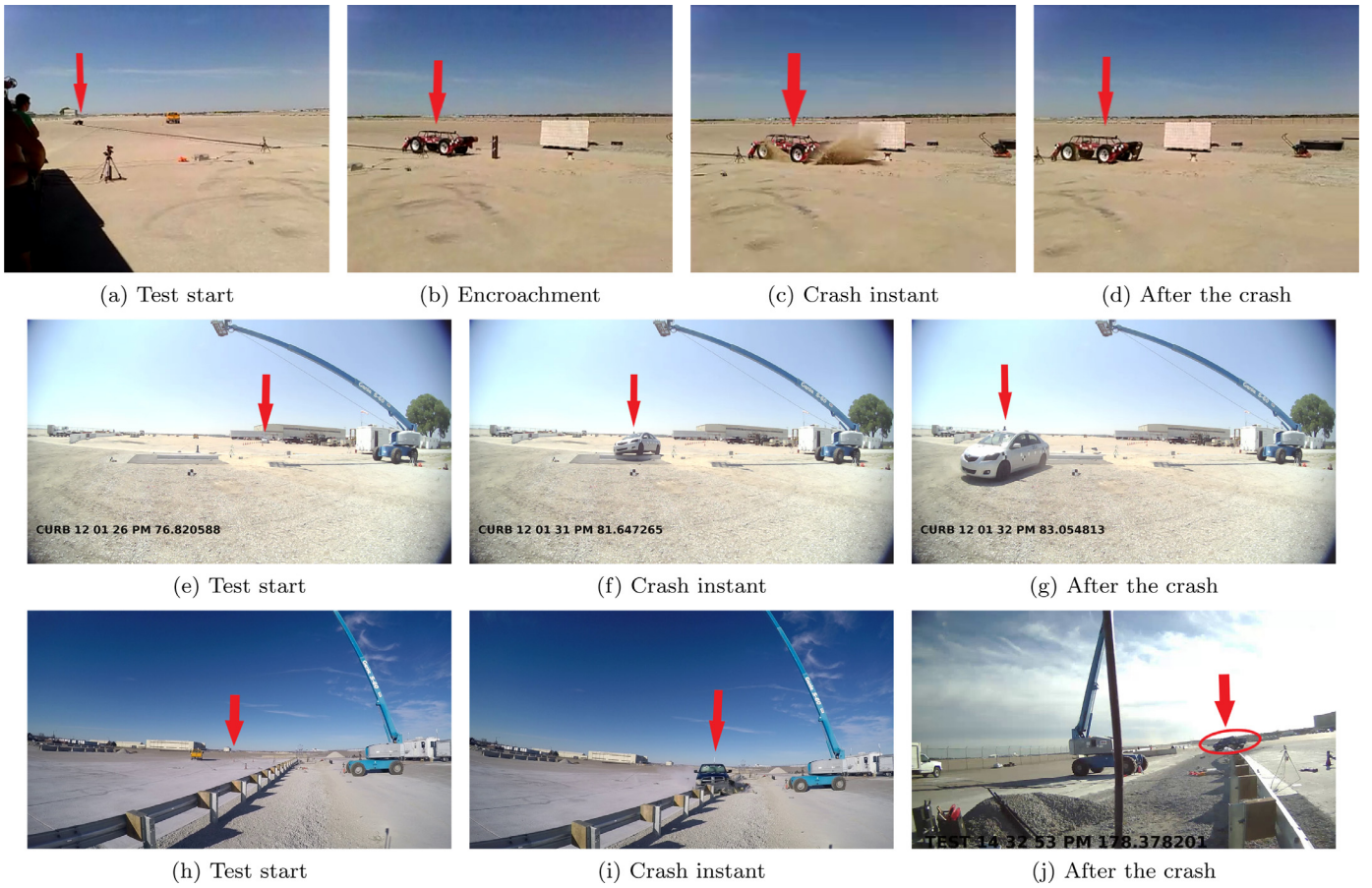
Fig. 6. Snapshots of different stages of crash tests: (a–d) Bogie, (e–g) Sedan, and (h–j) Pickup.
