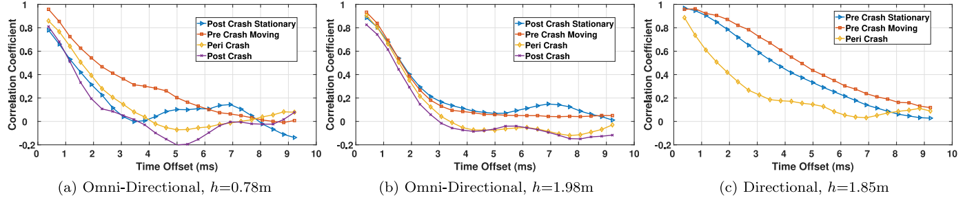
Fig. 22. Channel coherence of 4 intervals for lower and upper barrier antennas in pickup test.
