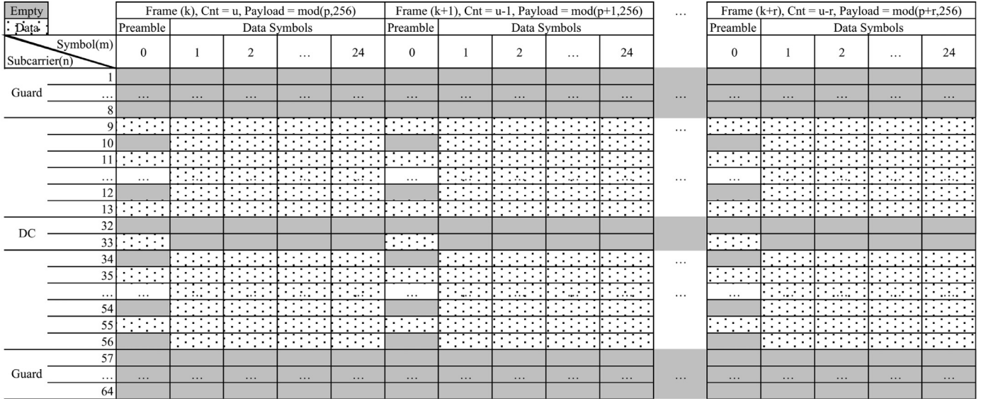
Fig. 7. OFDM frame structure for the experiments.
