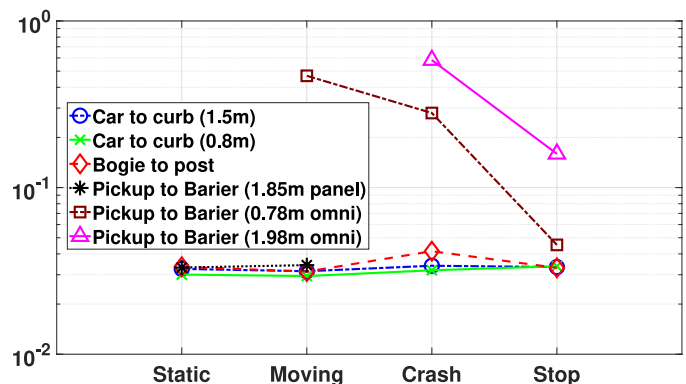
Fig. 24. BER of 4 phases in bogie and sedan crash tests.
