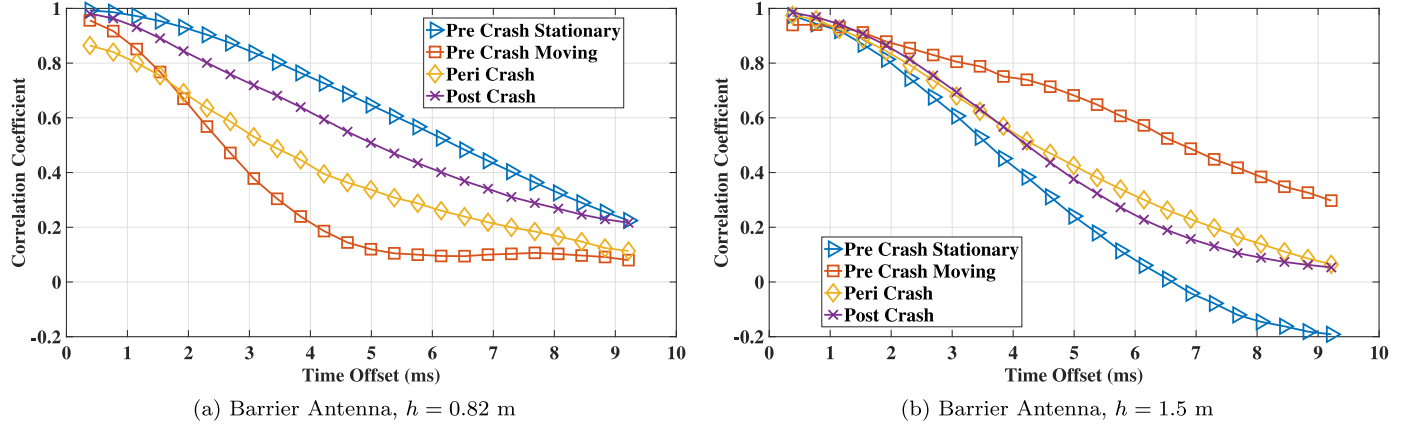
Fig. 16. Channel coherence in 4 intervals for lower and upper antennas in sedan test (a) h = 0.82 , (b) h = 0.82 m.
