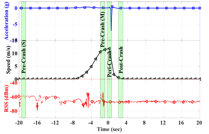
Fig. 8. Acceleration, velocity, and RSS in the bogie test, antenna height 0.9 m.
